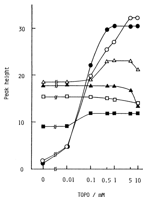
Fig. 4. Effect of TOPO concentration. Symbols and experimental conditions are identical to those shown in Fig. 1 and Table 1, respectively.
