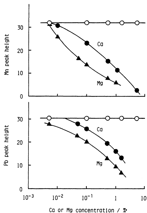
Fig. 2. Effect of Ca or Mg concentration on Mn and Pb absorption signals. Open symbols: 1 mM STTA-1 mM TOPO extraction. Closed symbols: 1 mM STTA-1 mM TOPO extraction.
