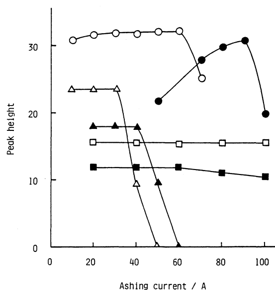
Fig. 1. Effect of ashing current on absorption signal of each metal. ○: Mn 40 ng, ●: Pb 125 ng, △: Cd 5 ng, ▲: Ni 300 ng, □: Cu 250 ng, ■: Co 100 ng.
