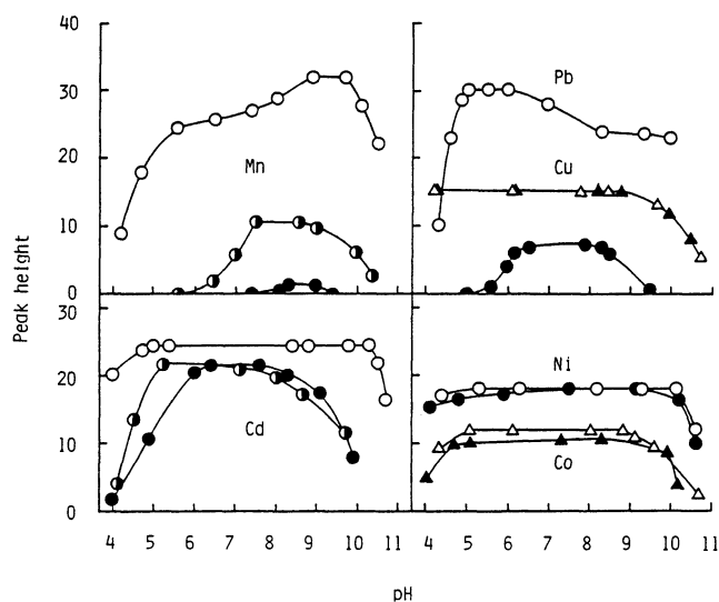
Fig. 3. Effect of extraction pH on absorption signals of each metal. Open and closed symbols denote the absorbances by STTA-TOPO and STTA extraction, respectively, except for STTA-TBP extraction (●). The reagent and metal concentrations are identical to those shown in Table 1 and Fig. 1, respectively.
